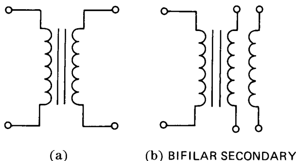
Figure 2—Pulse-Transformer Schematics
